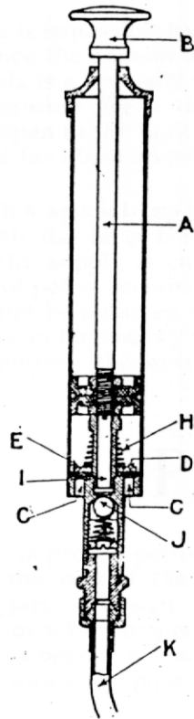
SECTION OF ARIEL OIL PUMP.
